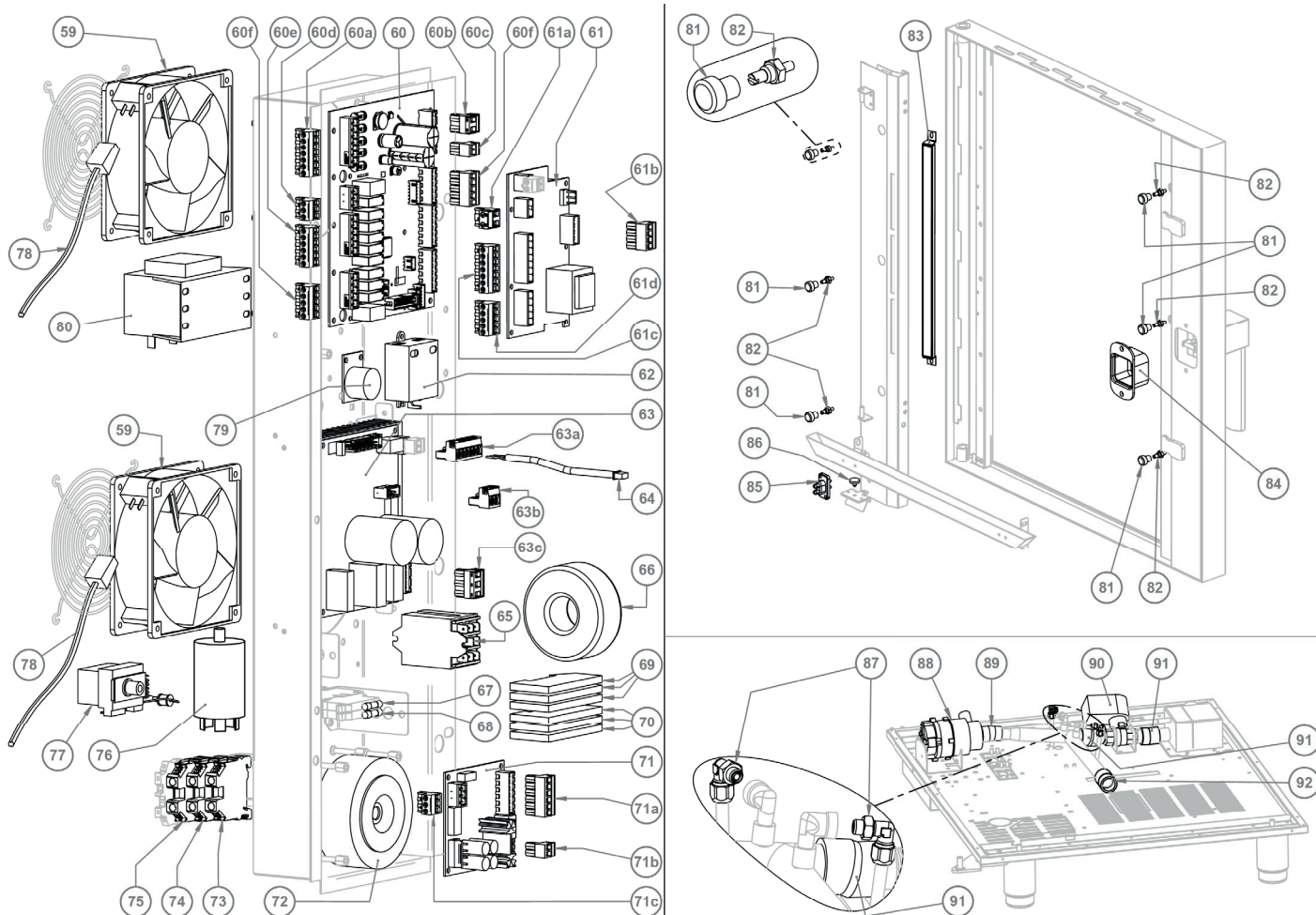
Exploded view 2/3
